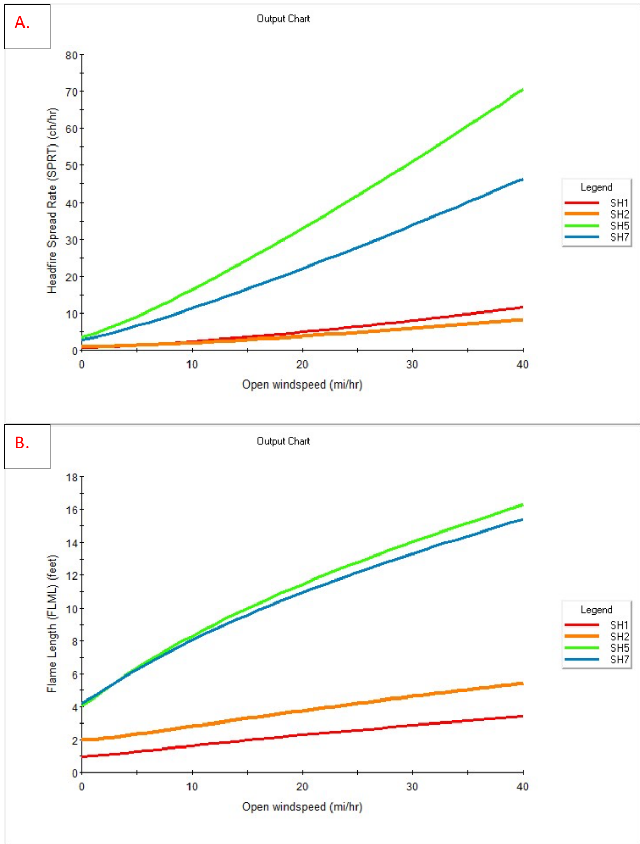
Figure 20. Simulated Rate of Spread (A) and Flame Length (B) for Shrub surface fuel models.
